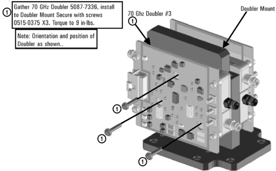
Figure 3 Installing A61 Doubler 3 on the Doubler Mount
