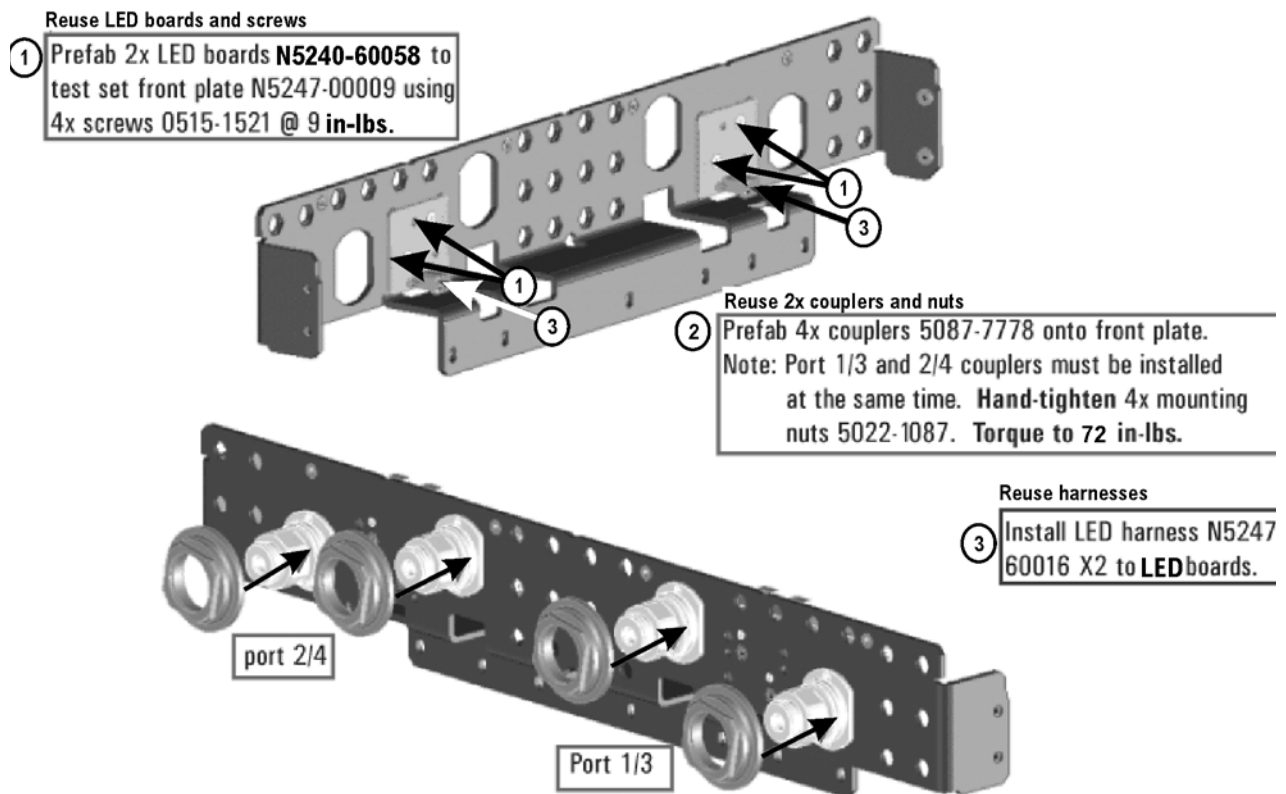
Figure 24 LED Board Assemblies and Test Port Coupler Assemblies Installation
