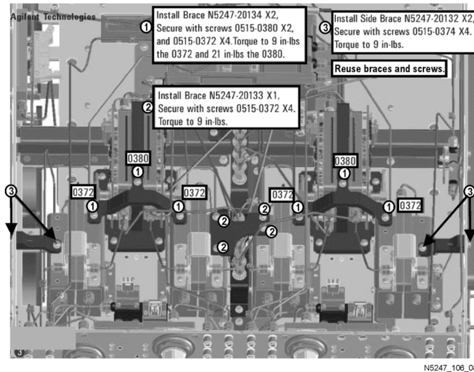
Figure 31 Location of Braces on the Bottom Side of the PNA
