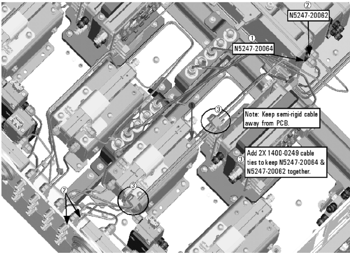
Figure 29 Location of Cable Ties to Secure W120/W54
