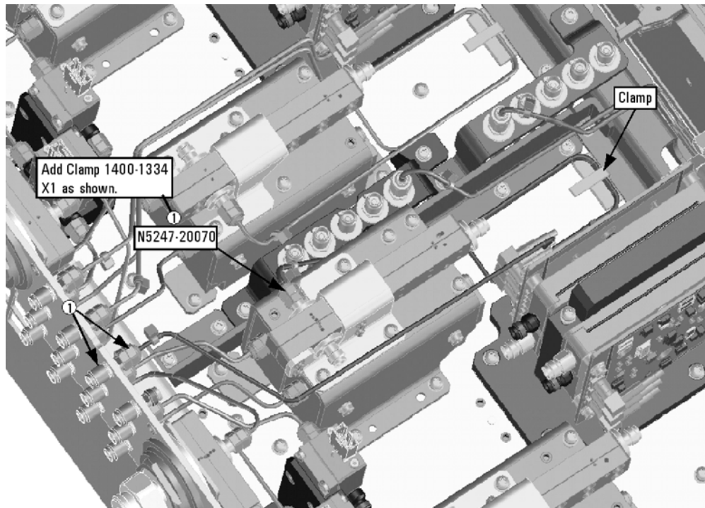
Figure 28 Location of Cable Clamp to Secure W37
