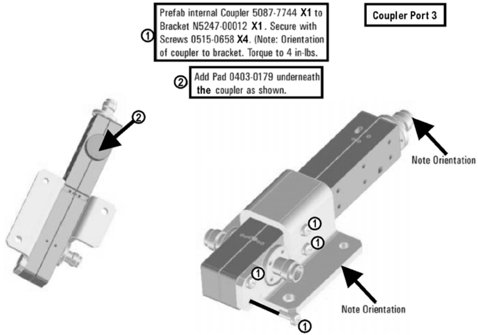
Figure 19 A30 receiver coupler Assembly
