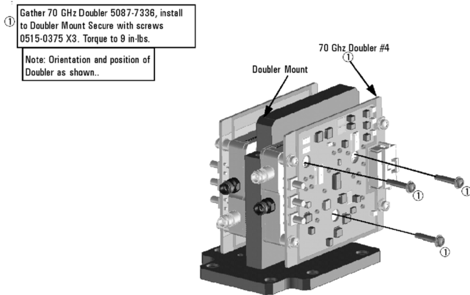
Figure 5 Installing A62 Doubler 4 on the Doubler Mount
