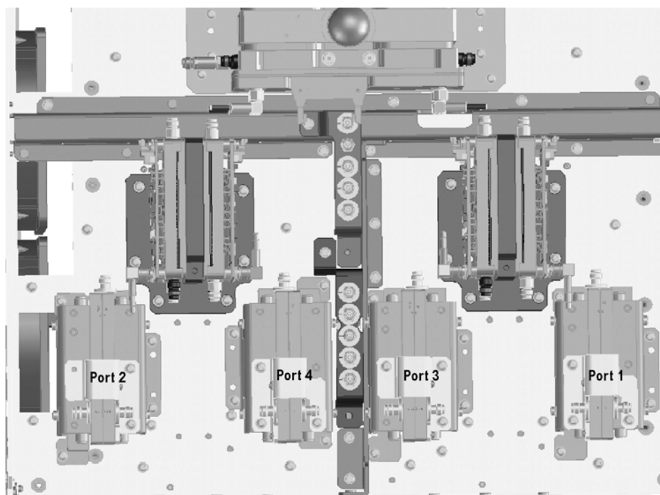
Figure 21 Location of Attenuator Assemblies and receiver coupler Assemblies
